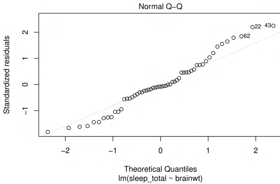
Figure 2: Linearity test Q-Q plot
